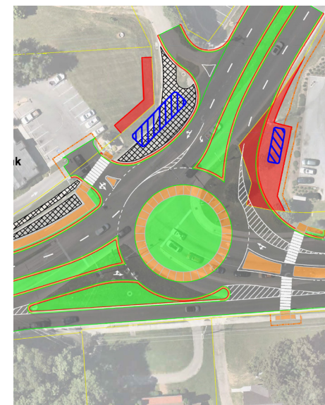
Roundabout engineering plan
